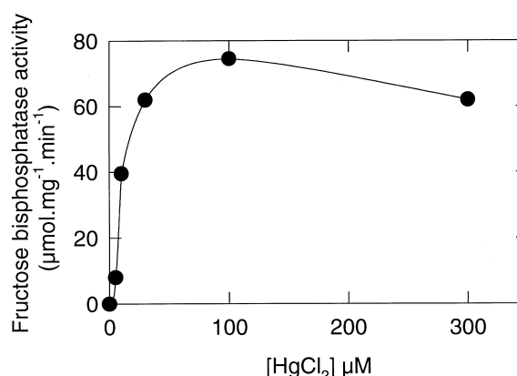
Fig. 1. Effect of \text{HgCl}_2 concentration on chloroplast fructose-1,6-bisphosphatase. Fructose-1,6-bisphosphatase activity was measured as described in Section 2 in assay mixtures containing 0.62 μg fructose-1,6-bisphosphatase and various concentrations of \text{HgCl}_2 .
